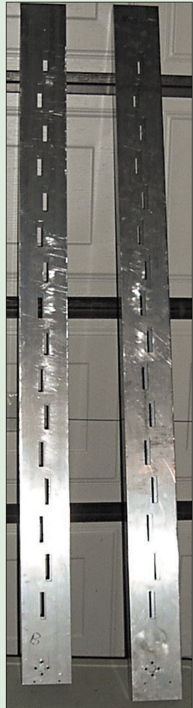
Figure A—The design of the slot antenna allows it to be easily reproduced with a milling machine.
